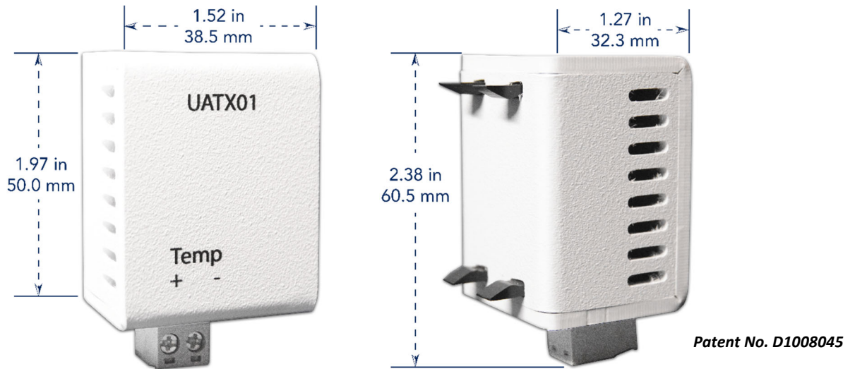
Figure 1 - Temperature Sensor with Dimensions
